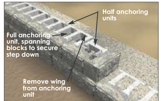
Install the half of an anchoring unit.
